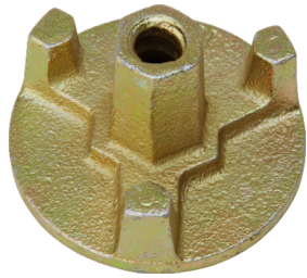
THREE WING ANCHOR NUT Material : SG Iron Size : 100mm Weight : 0.640 KG Working Load : 90 KN
