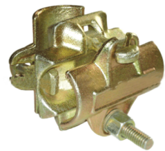
ITALIAN DOUBLE COUPLER FOR TUBE OD 48.3mm
