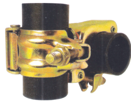
JAPANESE DOUBLE COUPLER FOR TUBE OD 48.3MM & 42.3MM (JIS : G3444 / SS-311)
