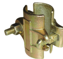
ITALIAN HALF COUPLER FOR TUBE OD 48.3mm
