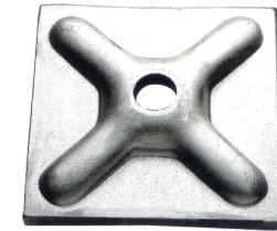
WALLER PLATE Material : S137 Size : 120x120x6/10mm Weight : 0.660 / 1.10 KG
