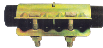
SLEEVE COUPLER FOR TUBE OD 48.3mm (EN-74 / BS-1139)
