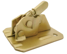
SPRING CLAMP Material : HR Sheet Size : Ø 4 - 10mm Weight : 0.460 kg
