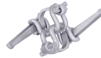
ROD TYPE DOUBLE COUPLER FOR TUBE OD 48.3mm
