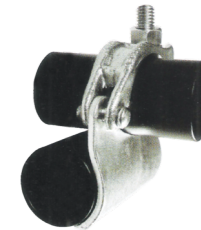
PULL LOG COUPLER FOR TUBE OD 48.3mm (EN-74 / BS 1139)
