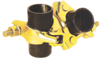
PRESSED SWIVEL COUPLER FOR TUBE OD 48.3mm (EN-74/BS-1139)
