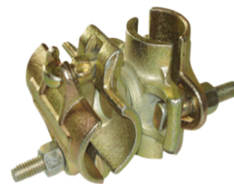
ITALIAN SWIVEL COUPLER FOR TUBE OD 48.3mm
