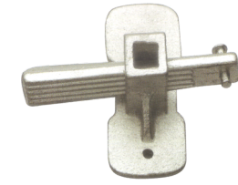
WEDGE CLAMP Material : High Quality Steel (Casted Body & Forged Wedge) Size : Ø 4 - 10mm / Ø 7 - 12mm Weight : 0.380 Kg / 0.490 Kg
