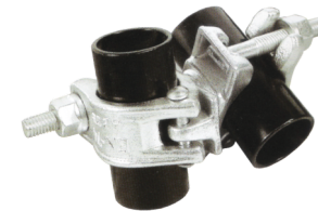
SWIVEL COUPLER GERMAN TYPE FOR TUBE OD 48.3mm (EN-74 / BS 1139)
