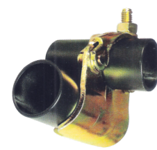
PRESSED PUTLOG COUPLER FOR TUBE OD 48.3mm (EN-74 / BS-1139)
