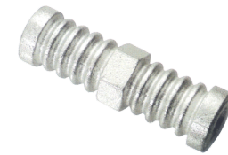
WATER BARRIER WITHOUT DISC Material : SG Iron Size : 120mm Length Weight : 0.500 KG
