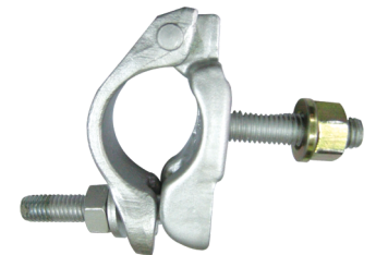
COUPLER WITH WELDED BOLT FOR TUBE OD 48.3mm
