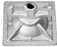
COMBINATION PLATE SQUARE (PLATE CASTED & NUT FORGED)
