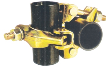
PRESSED DOUBLE COUPLER FOR TUBE OD 48.3mm (EN-74/BS-1139)
