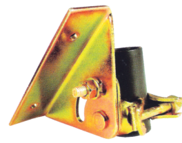
STAIRCASE COUPLER FOR TUBE OD 48.3mm (BS-1139)
