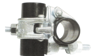
DOUBLE COUPLER GERMAN TYPE FOR TUBE OD 48.3mm (EN-74 / BS 1139)
